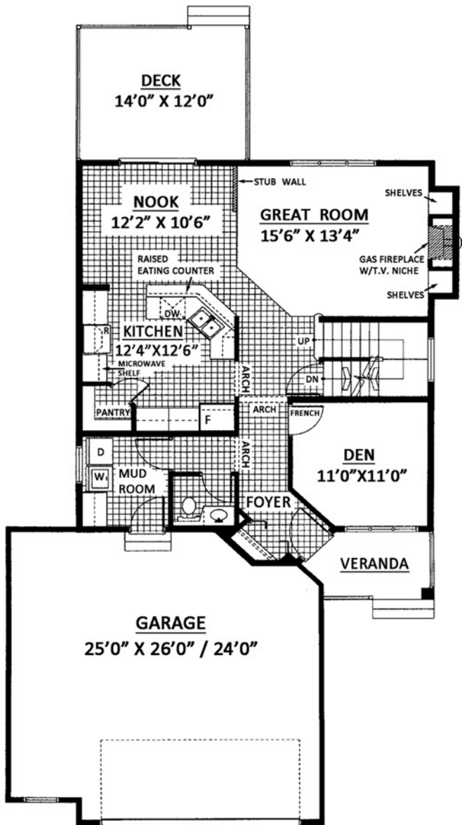
MAIN FLOOR PLAN 977 SQ. FT.
