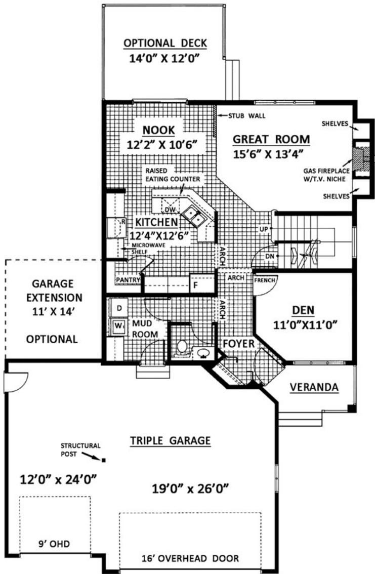
MAIN FLOOR PLAN 977 SQ. FT.
