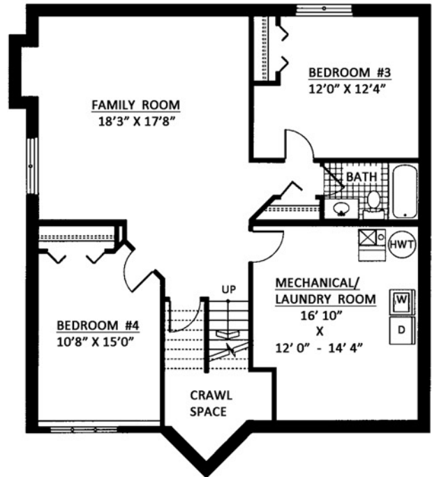
BASEMENT FLOOR PLAN 837 SQ. FT. PLUS MECHANICAL / LAUNDRY ROOM
